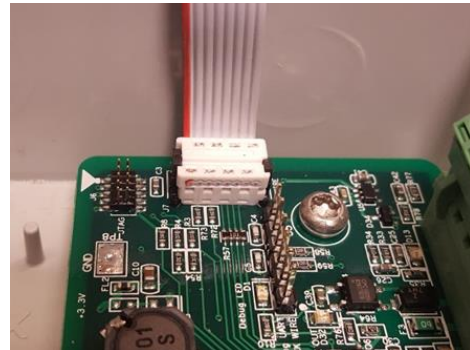
Connection of the wire to the bottom PCB.
