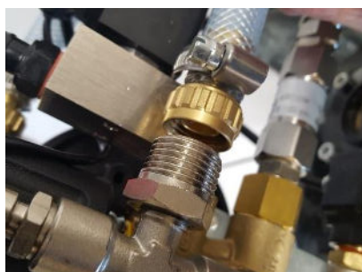
Demount the high-pressure pipe. Demount the by-pass hose
